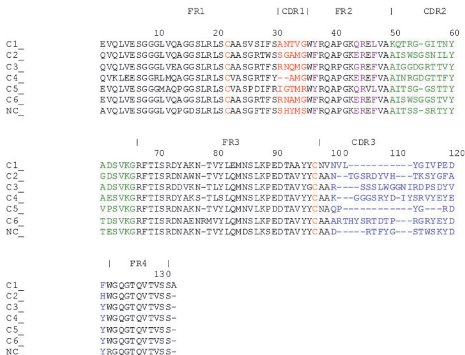
Fig. 1. Amino acid sequences of the six selected HBcAg-specific VHHs (C1–C6) and the non-HBcAg-specific VHH (NC). The framework regions (FR) and complementary determining regions (CDR) are indicated. CDR1 is highlighted in red, CDR2 in green and CDR3 in blue. Residues in purple represent residues that are characteristic for camelids. Residues in orange represent cysteines that can form disulphide bridges.
