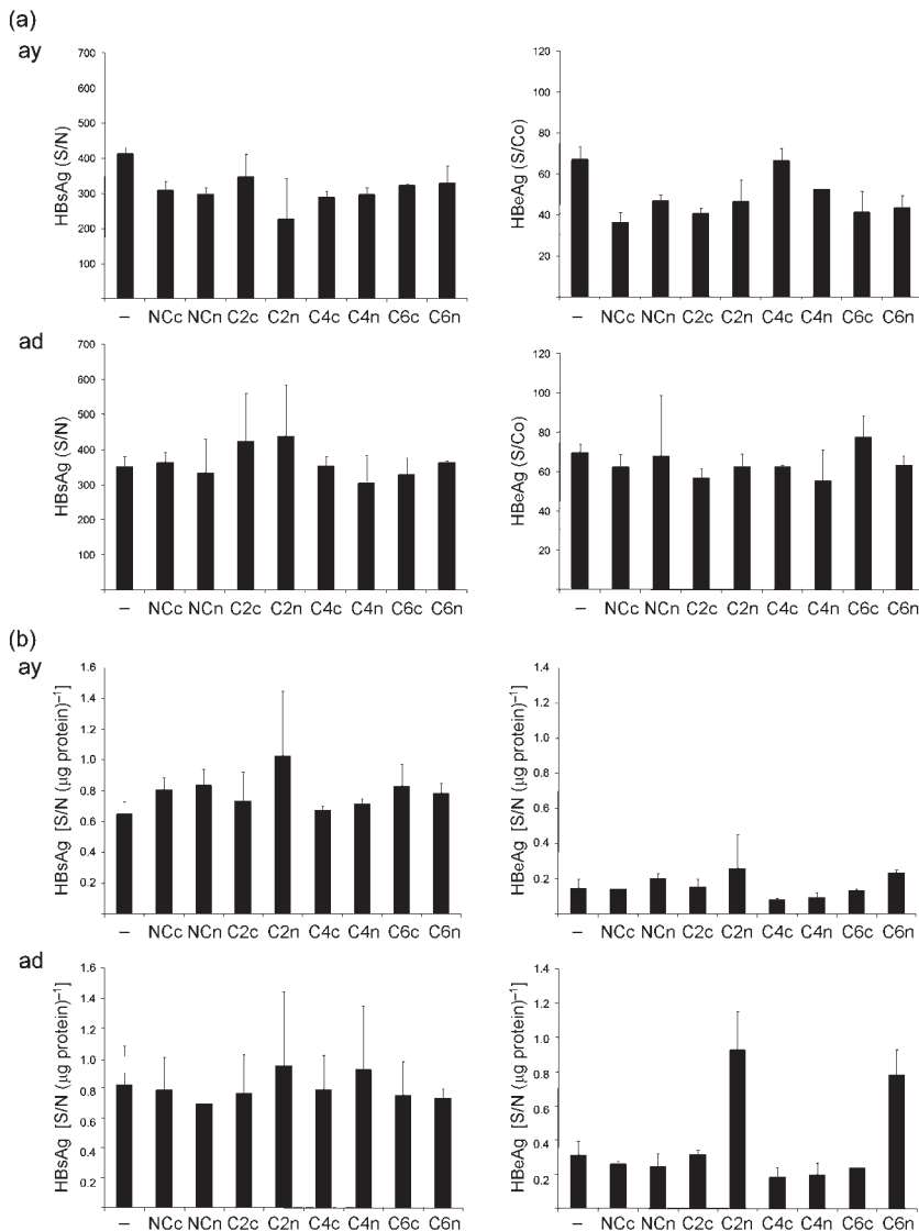
Fig. 5. Determination of HBsAg and HBeAg levels in cell culture medium (a) and cell lysate (b). HepG2 cells were transfected with 10 \mu g pSPayw1.3 or pSPadw1.3 plasmid, 2 \mu g VHH-pShooter vector and 8 \mu g empty pShooter plasmid (3 days post-electroporation). S/N, Signal-to-noise; S/Co, signal-to-cutoff.
