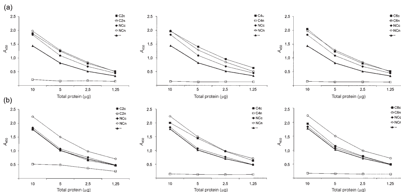
Fig. 6. Detection of intracellular HBcAg content in cells cotransfected with 10 µg pSPayw1.3 (a) or pSPadw1.3 (b) plasmid, 2 µg VHH-pShooter vector and 8 µg empty pShooter plasmid (3 days post-electroporation). The presence of HBcAg in HBcAg-specific VHH-transfected cells was compared with transfections without VHH (–) or with the non-HBcAg-specific VHH NC.
