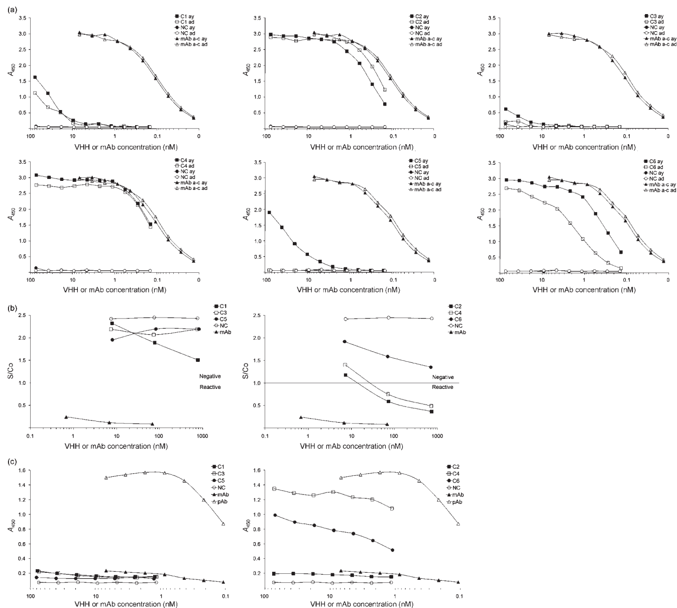
Fig. 2. Binding characteristics of the HBCAg-specific VHs (C1–C6), the non-HBCAg-specific VHH NC as negative control and a monoclonal mouse anti-HBCAg antibody as a positive control. (a) Study of the binding of the E. coli -purified VHH molecules on HBCAg subtypes ayw and adw by a VHH-binding ELISA. (b) Detection of anti-HBCAg activity by AxSYM CORE. (c) Binding of the VHH molecules on 1 \mu\text{g ml}^{-1} coated HBeAg. A monoclonal (mAb) and a polyclonal (pAb) anti-core antibody were included as control antibodies.
